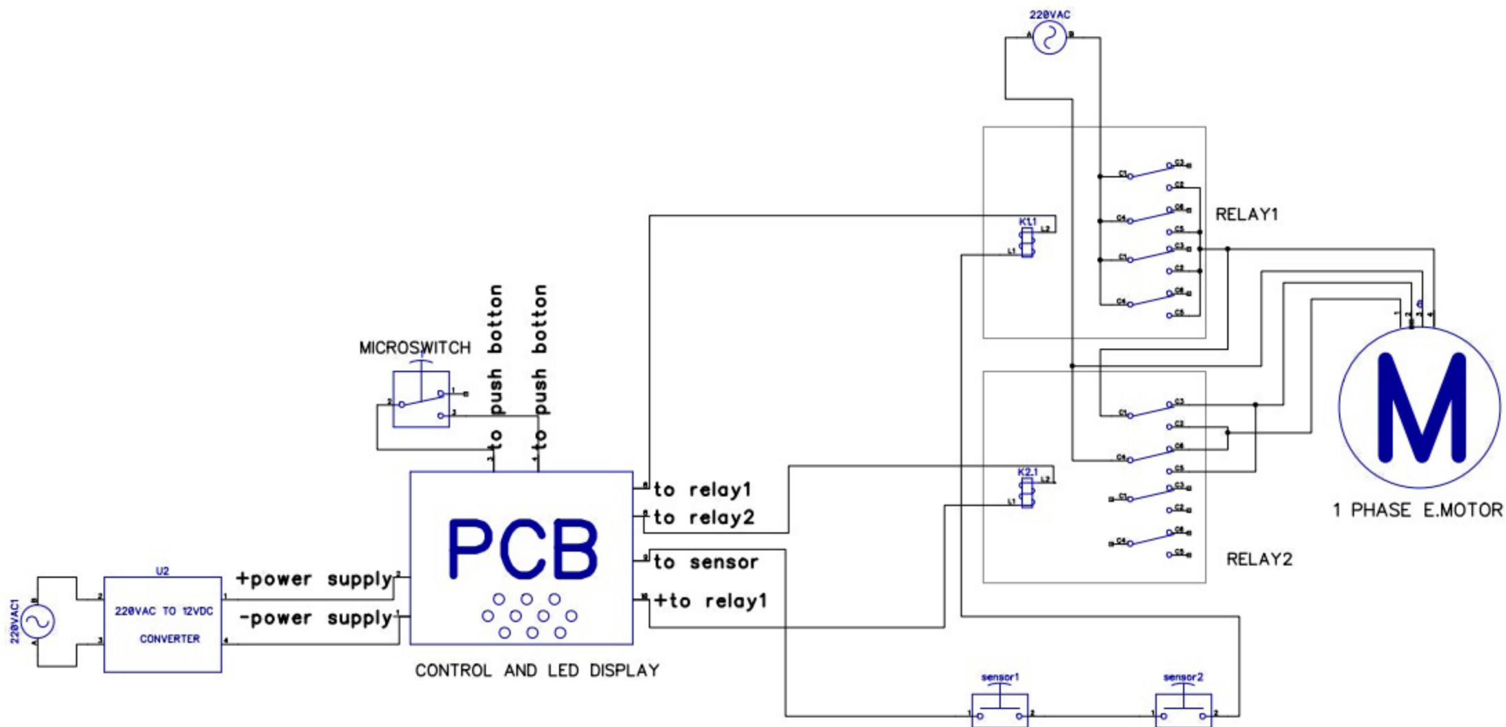
ELECTRIC SCHEM
